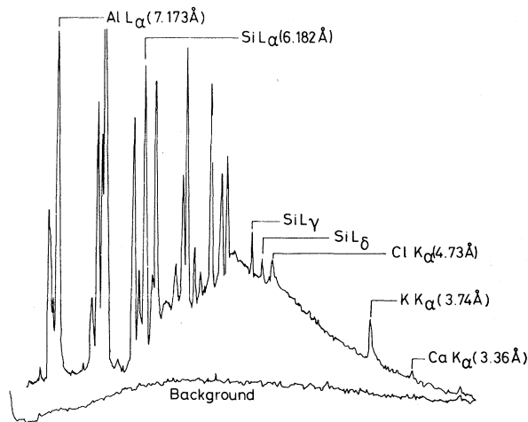
FIG. 1. A typical microdensitometer tracing from the front spectrometer. The Ca K\alpha line appears much more brightly on the rear spectrometer, where it suffers no target absorption.
