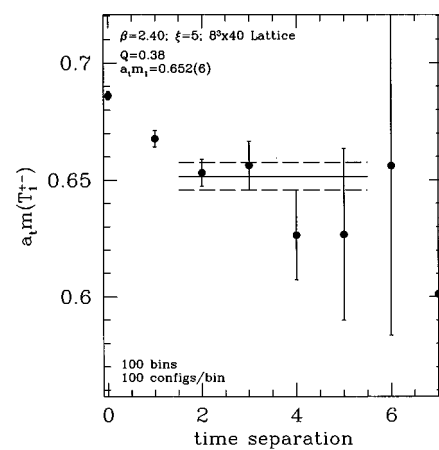
FIG. 9. Effective mass plot showing the results of a single-exponential fit to the glueball correlation function for the T_1^{+-} channel for \beta=2.4 and \xi=5 .
