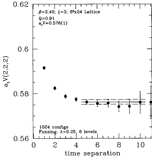
FIG. 2. Effective mass plot showing the results of a single-exponential fit to the Wilson loop for V(\vec{r}) with \vec{r}/a_s=(2,2,2) , \beta=2.4 , and \xi=3 . The t_{\min}-t_{\max} region of the fit is also indicated.
