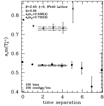
FIG. 11. Effective mass plot showing the results of a two-exponential fit to the 2 \times 2 matrix of glueball correlation functions for the T_2^{++} channel for \beta=2.4 and \xi=5 . The t_{\min}-t_{\max} region of the fit is also indicated.
