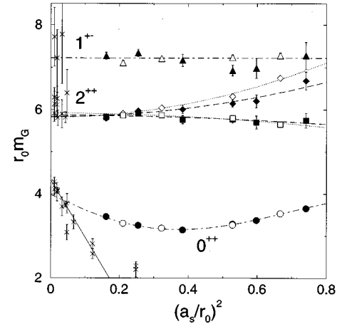
FIG. 12. Glueball mass estimates in terms of r_0 against the lattice spacing (a_s/r_0)^2 . Results from the \xi=5 simulations for the lattice irreps A_1^{++} , E^{++} , T_2^{++} , and T_1^{+-} are labeled \circ , \square , \diamond , and \triangle , respectively. The corresponding solid symbols indicate the results from the \xi=3 simulations. Data from Wilson action simulations taken from Refs. [19–22] are shown using crosses. The dashed, dotted, and dash-dotted curves indicate extrapolations to the continuum limit obtained by fitting to the \xi=3 data, the \xi=5 data, and all data, respectively. The solid line indicates the extrapolation of the Wilson action data to the continuum limit.
