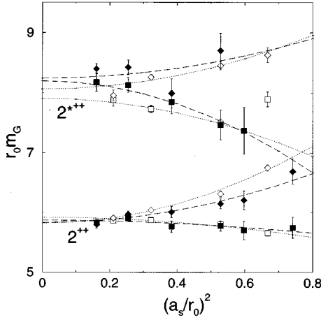
FIG. 13. Estimates of the masses of the tensor glueball and its first-excited state in terms of r_0 against the lattice spacing (a_s/r_0)^2 . Results from the \xi=5 simulations for the E^{++} and T_2^{++} irreps are labeled by \square and \diamond , respectively. The corresponding solid symbols show the results from the \xi=3 simulations. The dashed and dotted curves indicate extrapolations to the continuum limit obtained by fitting to the \xi=3 and the \xi=5 data, respectively (see Tables XVII and XVIII).
