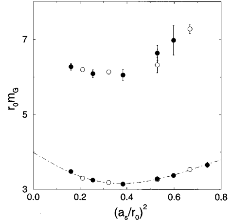
FIG. 14. Masses of the scalar glueball and its first-excited state in terms of r_0 against the lattice spacing (a_s/r_0)^2 . Open and solid symbols indicate results from the \xi=5 and \xi=3 simulations, respectively. The extrapolation to the continuum limit is indicated by the dash-dotted curve.
