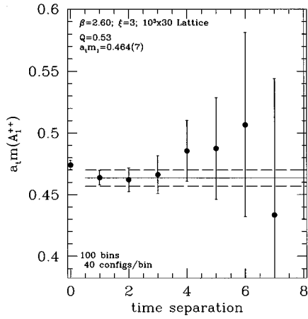
FIG. 4. Effective mass plot showing the results of a single-exponential fit to the glueball correlation function for the A_1^{++} channel for \beta=2.6 and \xi=3 . The t_{\min}-t_{\max} region of the fit is also indicated.
