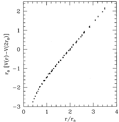
FIG. 3. The static-quark potential V(\vec{r}) expressed in terms of the hadronic scale r_0 . This plot includes measurements from the \beta=2.2, 2.4 , and 2.6 simulations for \xi=3 , and the \beta=2.2 and 2.4 simulations for \xi=5 . Lattice spacing errors are seen to be small.
