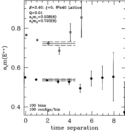
FIG. 10. Effective mass plot showing the results of a two-exponential fit to the 2 \times 2 matrix of glueball correlation functions for the E^{++} channel for \beta=2.4 and \xi=5 . The t_{\min}-t_{\max} region of the fit is also indicated.
