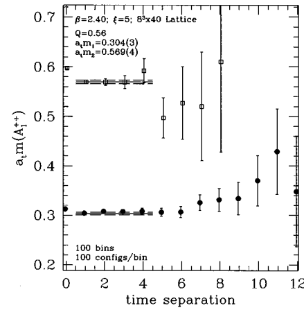
FIG. 8. Effective mass plot showing the results of a two-exponential fit to the 2 \times 2 matrix of glueball correlation functions for the A_1^{++} channel for \beta=2.4 and \xi=5 . The t_{\min}-t_{\max} region of the fit is also indicated.
