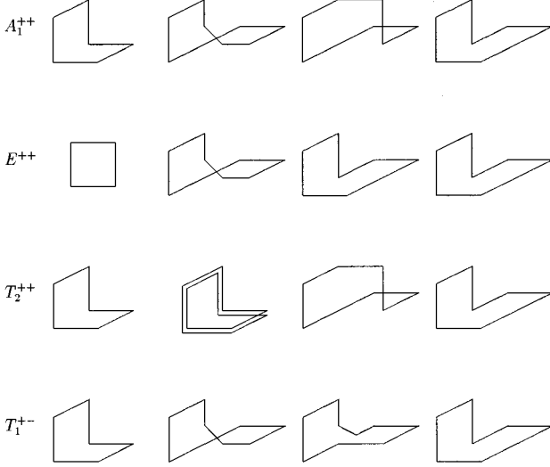
FIG. 1. The four Wilson loop shapes in each channel used to form the lattice glueball operators. The complete set of 24 operators was formed by computing linear combinations of each of these loops rotated and translated across the lattice on six different sets of smoothed links. Where a loop shape occurs twice, it is used in two different projections into the appropriate irreducible representation.
