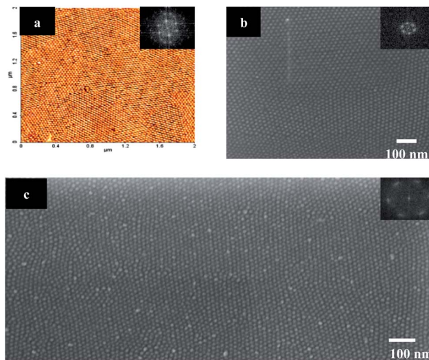
Fig. 7 AFM topography image (a), top-down high resolution SEM image (b) of iron oxide nanodots obtained after UV/Ozone treatment for 3 h. (c) The iron oxide nanodot patterns obtained from the UV/Ozone treated film after calcination at 800 °C for 1 h.
