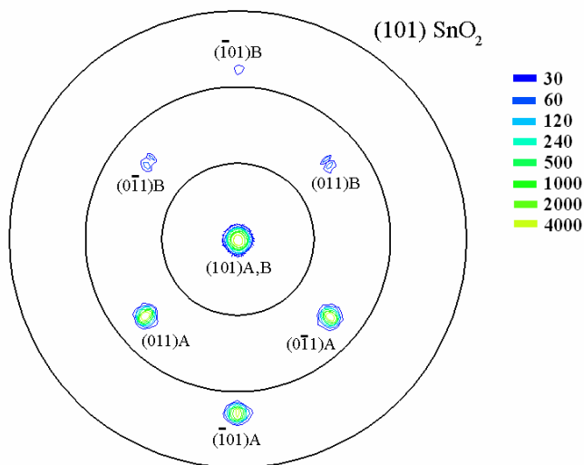
FIG. 6. (Color online) Pole figure of the \{101\} family of planes for a thin film of (\text{Sn}_{0.96}\text{Cr}_{0.04})\text{O}_2 .
