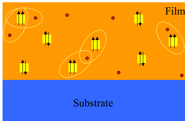
FIG. 15. (Color online) Illustration of the stabilization of two-electron/hole triplet states by coupling with magnetic dopant cations.
