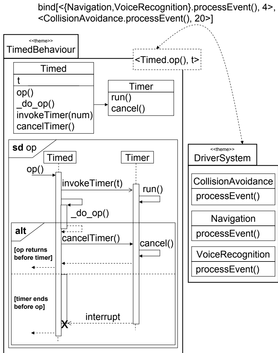
Figure 1. Separation of the timing concern in the driver information system using Theme/UML
