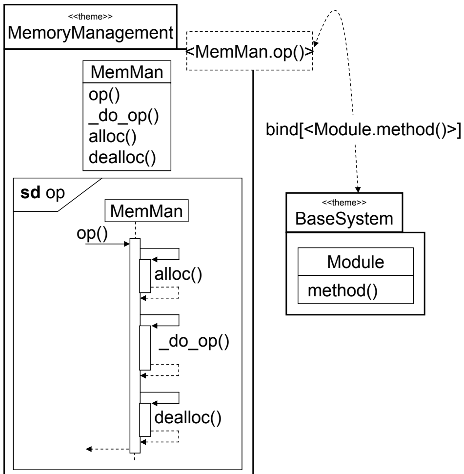
Figure 2. Separation of the memory management concern with Theme/UML
